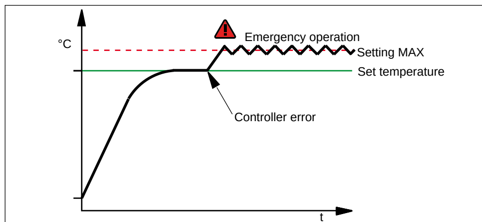
Fig. 21 Schematic diagram of how TWW temperature monitoring works
