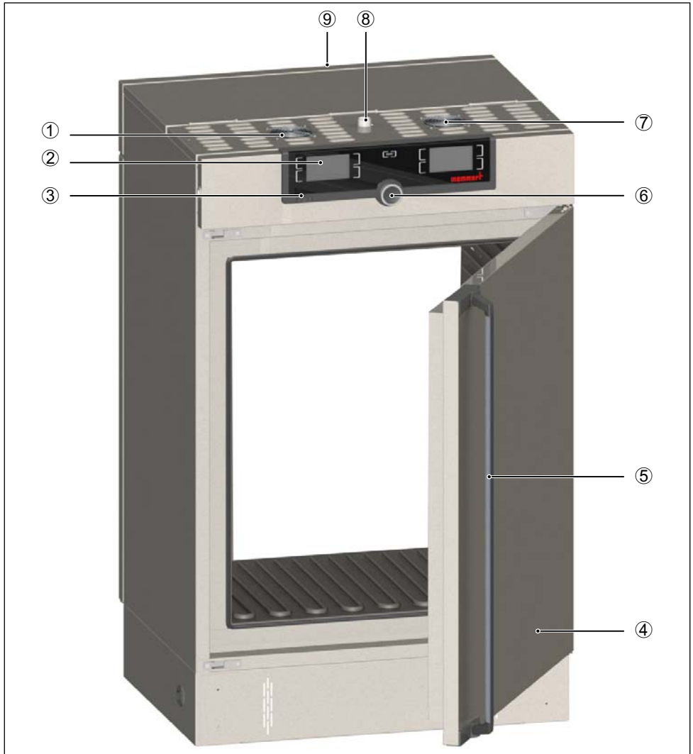
Fig. 2 Construction
