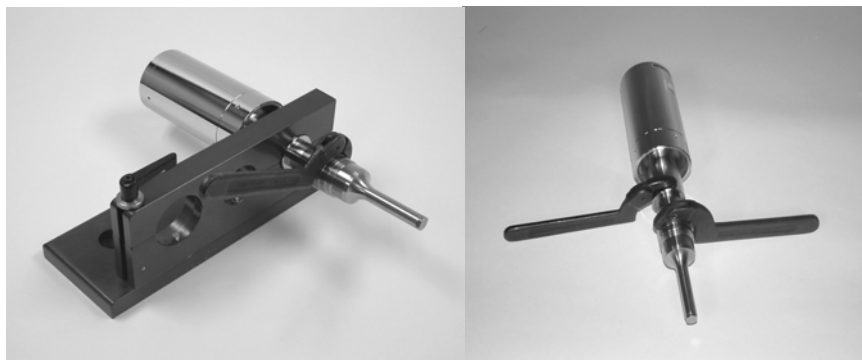
Figure 4.1 Methods For Connecting/Removing Horn From Converter
