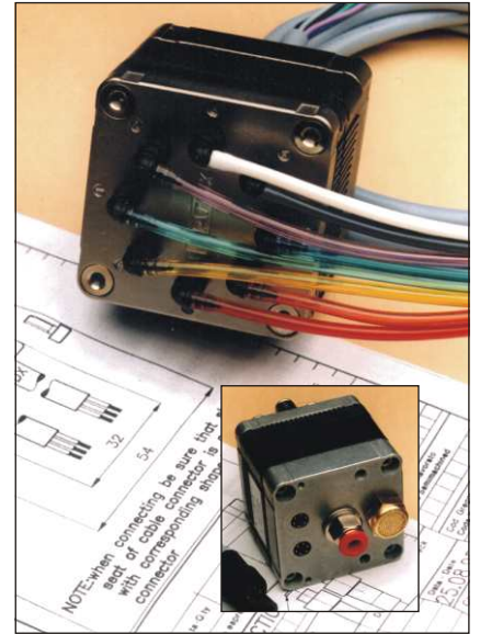
8 Way High Speed Sol Valve
